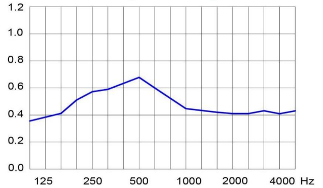
Absorption according to EN ISO 354
